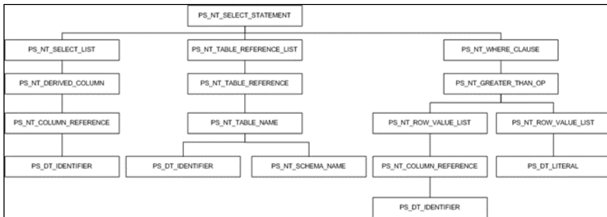
Figure 2 - Example Parse Tree for SELECT column1 from table1 where column1 > 0 with null nodes removed.
